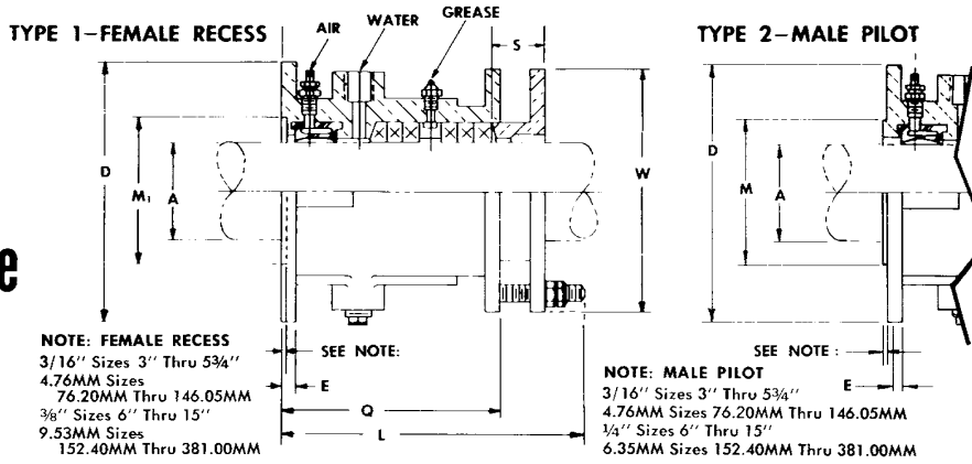
(FIG. 1786IR AIR WATER-GREASE SERVICE)
