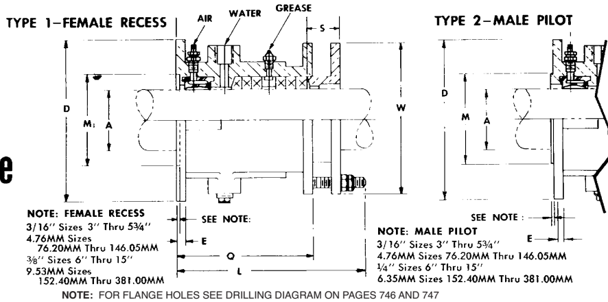
(FIG. 1786 IR AIR WATER-GREASE SERVICE)
